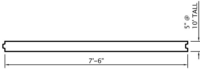
PLAN VIEW OF TOP
