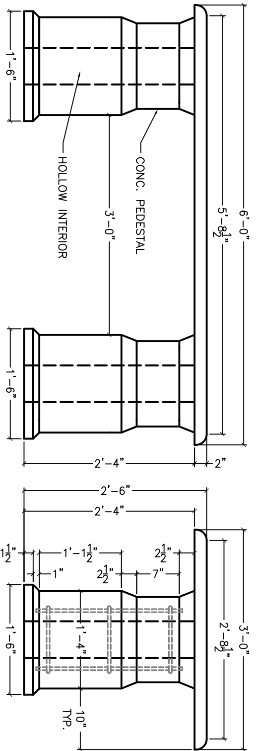
SIDE VIEW
